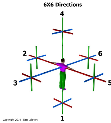
3D representation of the six lines.
